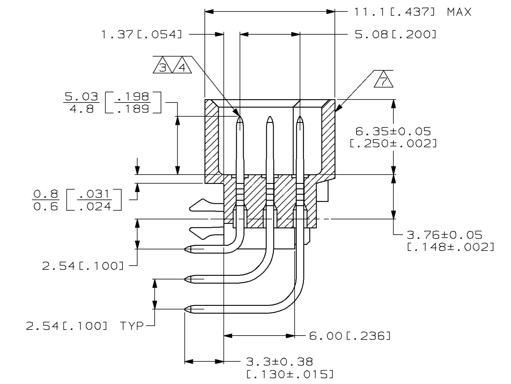
SECTION X-X
